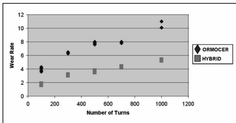
Fig. 8: Wear rate graph ( \text{mm}^3/\text{N}\cdot\text{mm} ) of ormocer (Admira) and hybrid composite (Concept) in cycles of 100, 300, 500, 700 and 1000 turns using aluminum dispersion.
