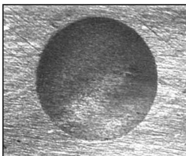
Fig. 5: Optic microscopy of the ormocer surface after 500 turns, after wear with aluminum dispersion.
