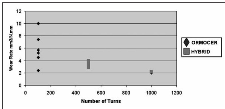
Fig. 6: Wear rate graph ( \text{mm}^3/\text{N}\cdot\text{mm} ) of ormocer and hybrid composite using diamond paste as abrasive.
