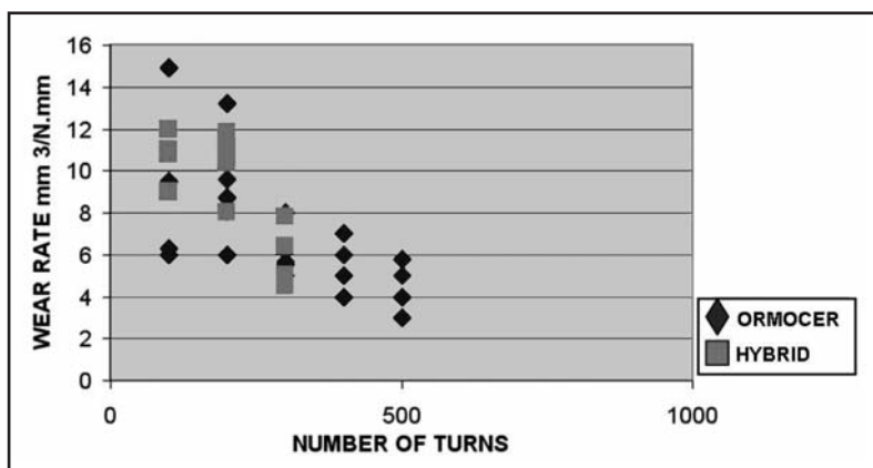
Fig. 7: Ormocer wear rate ( \text{mm}^3/\text{N}\cdot\text{mm} ) with cycle of 500 turns.
