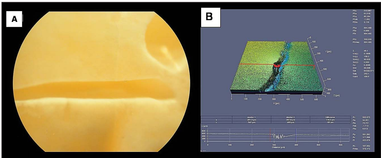
Fig. 1: A and B Groove-shaped enamel defects 200-400 µm deep and 100- 260 µm wide were created in the mesiodistal direction. Defect profiles and dimensions were established using stereomicroscope and confocal laser microscope.
